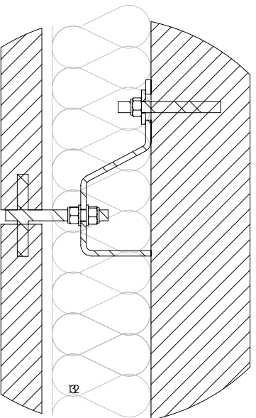
DETAIL B SCALE 1 : 5
